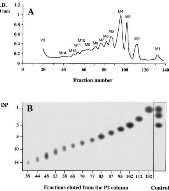
Fig. 1. Fractionation of the acid-labile oligomannosides of C. albicans strain NIH A 207. A: Gel filtration on a Biogel P2 column. V0: void volume; M1 to M14: degree of polymerization of the eluted oligomannosides. B: Thin layer chromatography of the fractions which correspond to the top of the peaks eluted on the Biogel P2; Solvent system: n -butanol/acetic acid/water (20/10/15); 5 µl of these fractions was spotted on Silicagel Si 60 except for fractions 103, 112 (2 µl) and 38, 43, 48 (8 µl). Mannose, saccharose and raffinose were used as controls. DP: degree of polymerization.
